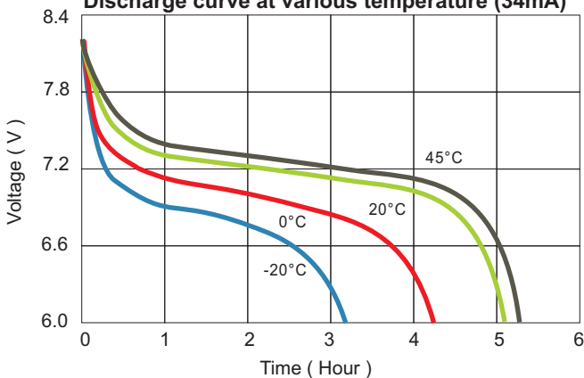
Discharge curve at various temperature (34mA)
